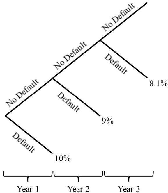
Figure 11.2A. Illustration of the default process through time assuming a conditional default probability of 10% per year.
