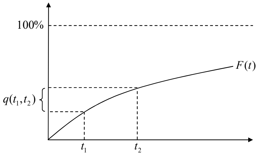
Figure 11.1A. Illustration of cumulative default probability function, F(t) , and marginal default probability, q(t_1, t_2) .
